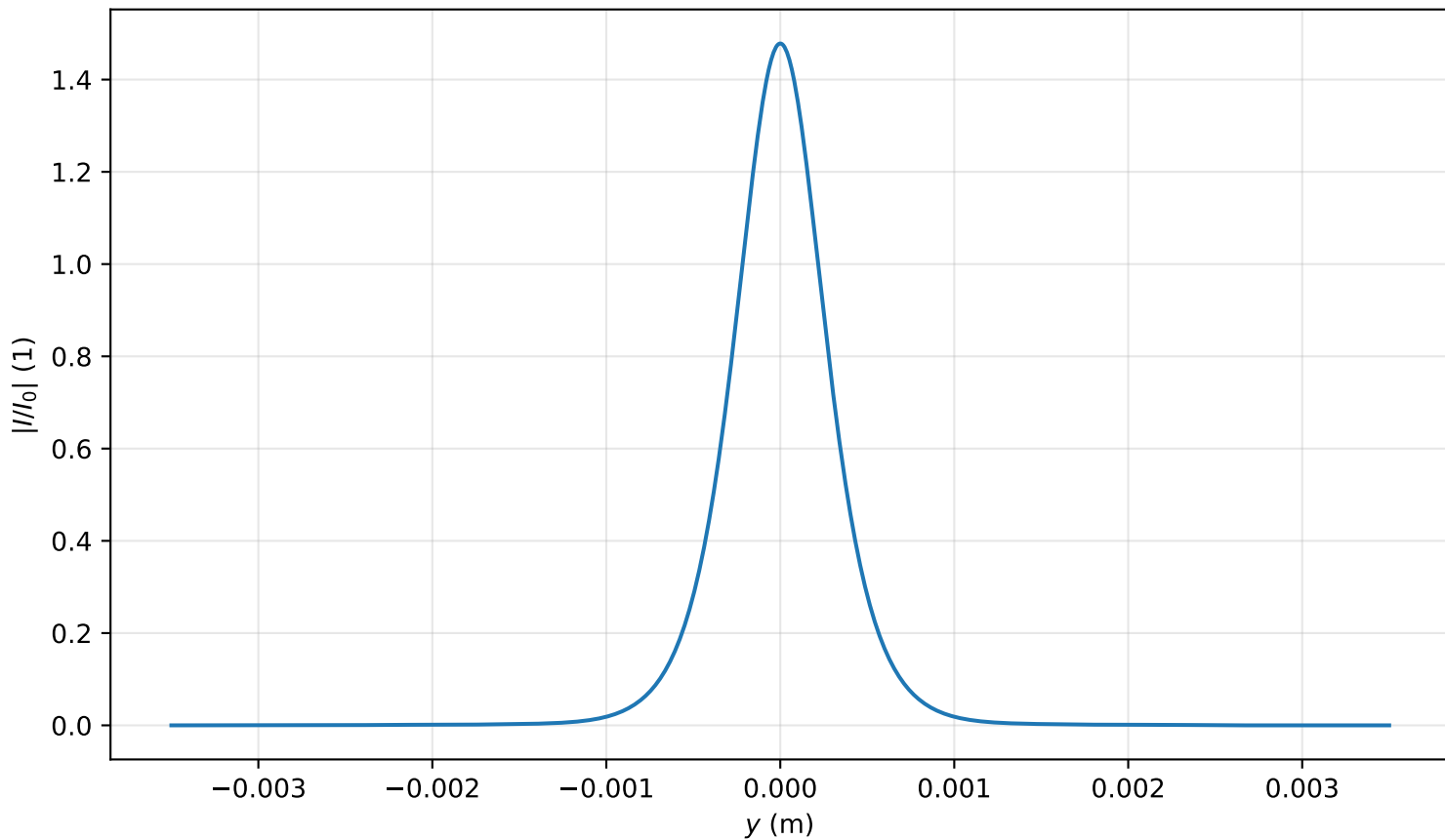
Intensity profile I(x=0, y, z=3.582)/I_0 , P_{in}=0.9P_{cr} , artificial time
